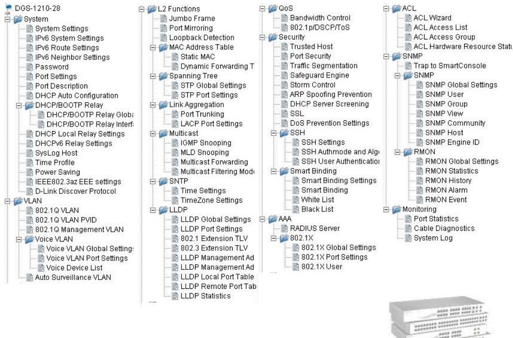
Figure 4.16 –Function Tree
