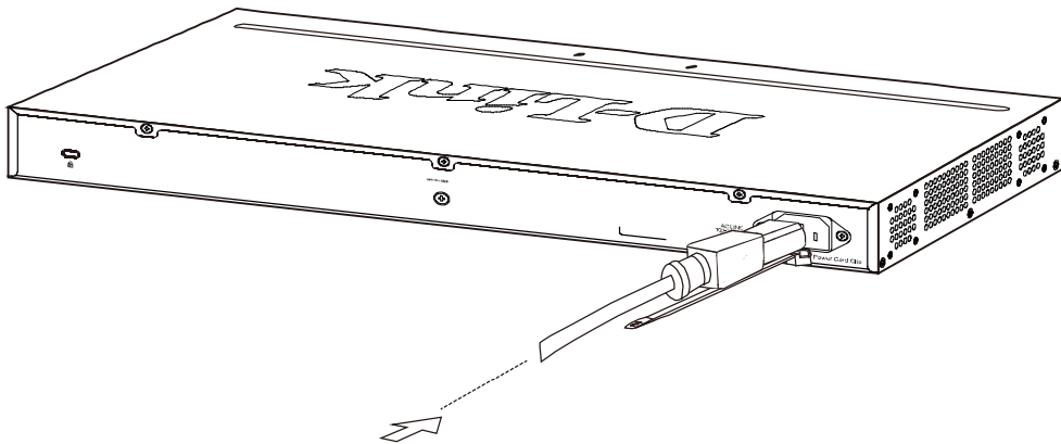
Figure 2.5 – Connect the power cord to the Switch
