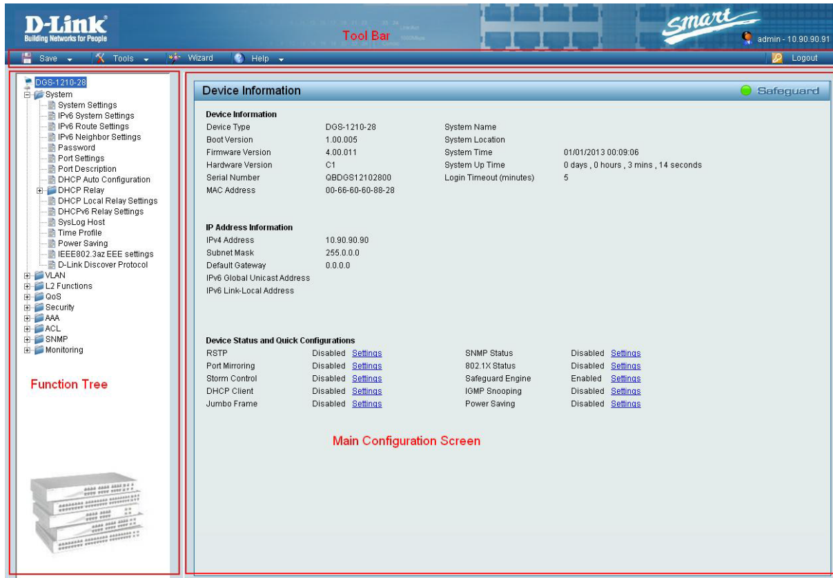
Figure 4.5 – Web-based Management
