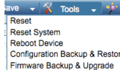
Figure 4.9 – Tool Menu
