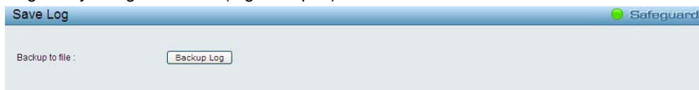
Figure 4.8 – Save Log
