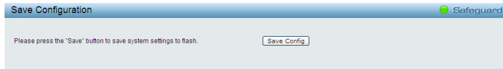
Figure 4.7 – Save Configuration
