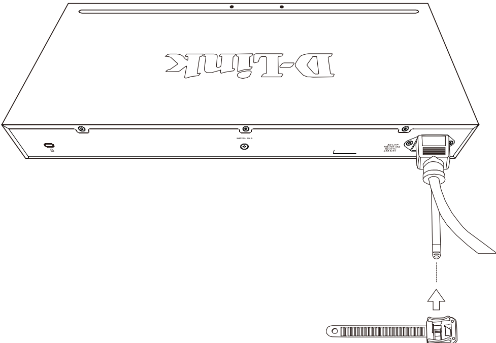
Figure 2.6 – Slide the Retainer through the Tie Wrap
