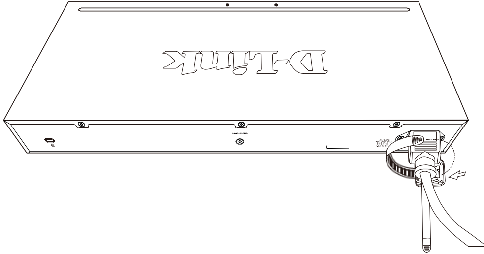
Figure 2.7 – Circle around the power cord
