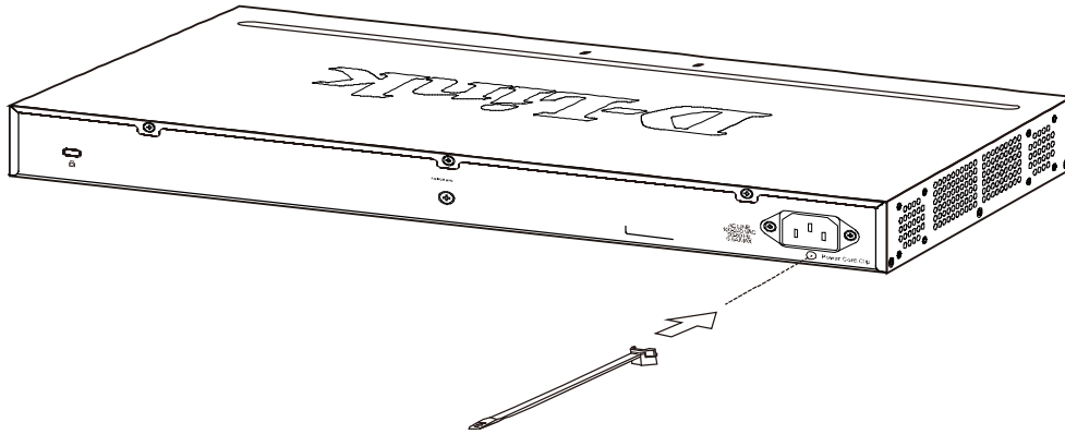
Figure 2.4 – Insert Tie Wrap to the Switch
